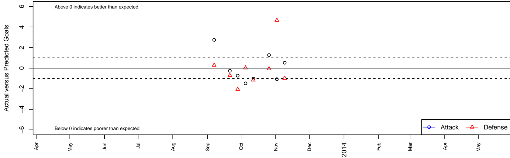
Nortac Arsenal B01 Dots are actual minus expected GF (blue circles) and GA (red triangles). Blue line is smoothed change in attack strength. Red is smoothed change in defense strength.
